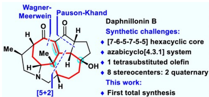
Scheme 3. Total Synthesis of (±)-Daphnillonin B
