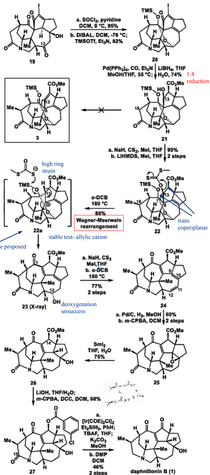
Scheme 3. Total Synthesis of (±)-Daphnillonin B
