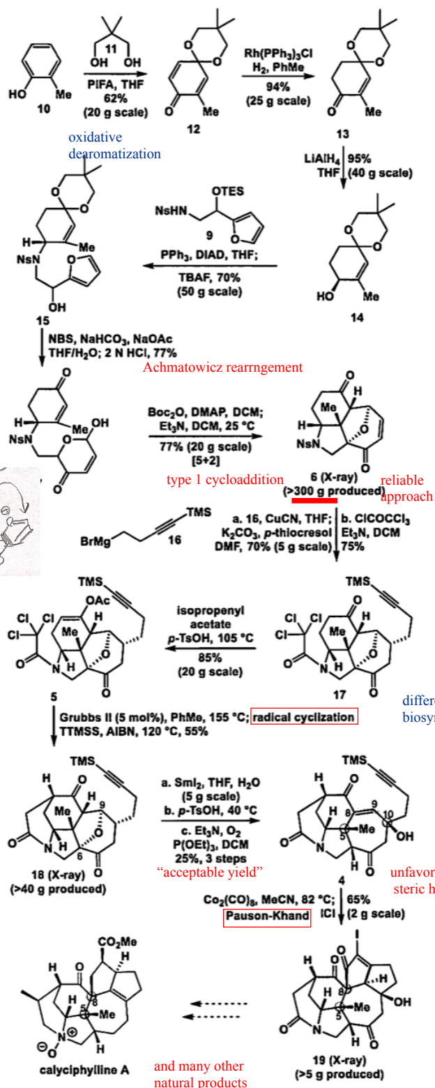
Scheme 2. Synthesis of Hexacyclic Core 19
