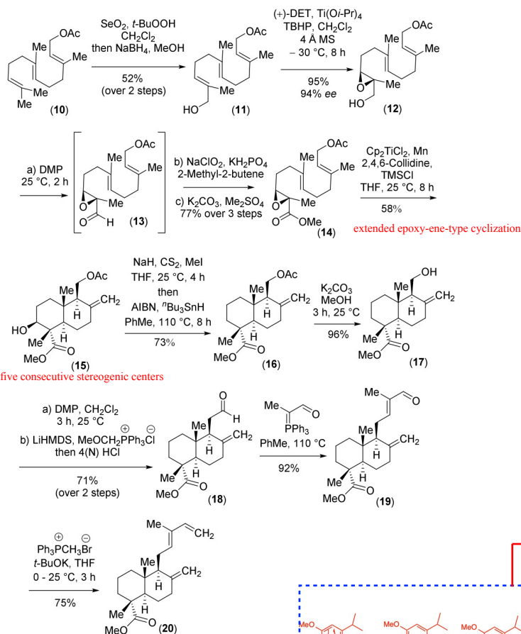
Scheme 2. Asymmetric Synthesis of trans -Ozic Acid Methyl Ester
