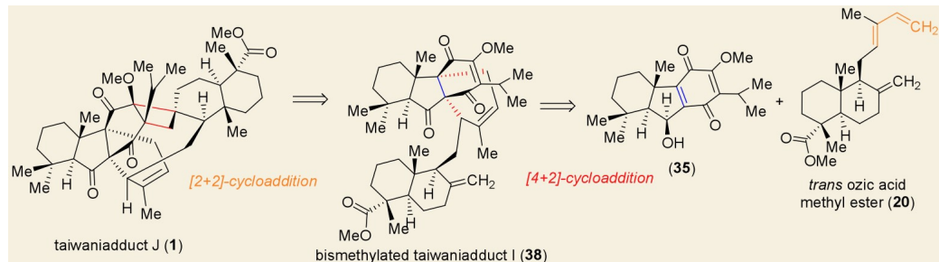
Scheme 3. Asymmetric Synthesis of abeo -Abietane Diterpenoid
