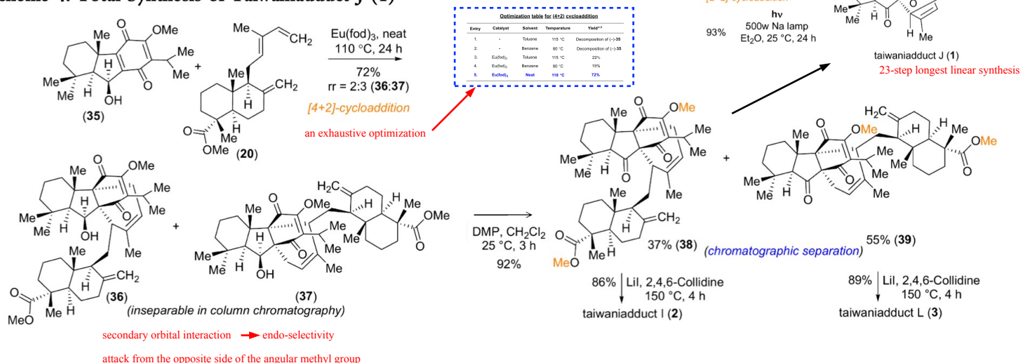
Scheme 4. Total Synthesis of Taiwaniadduct J (1)
