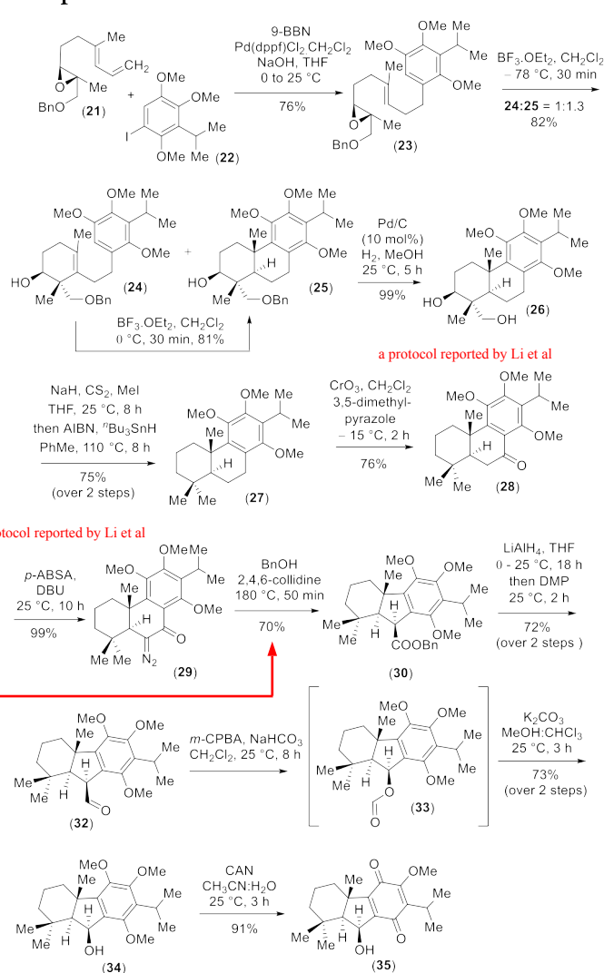
Scheme 3. Asymmetric Synthesis of abeo -Abietane Diterpenoid
