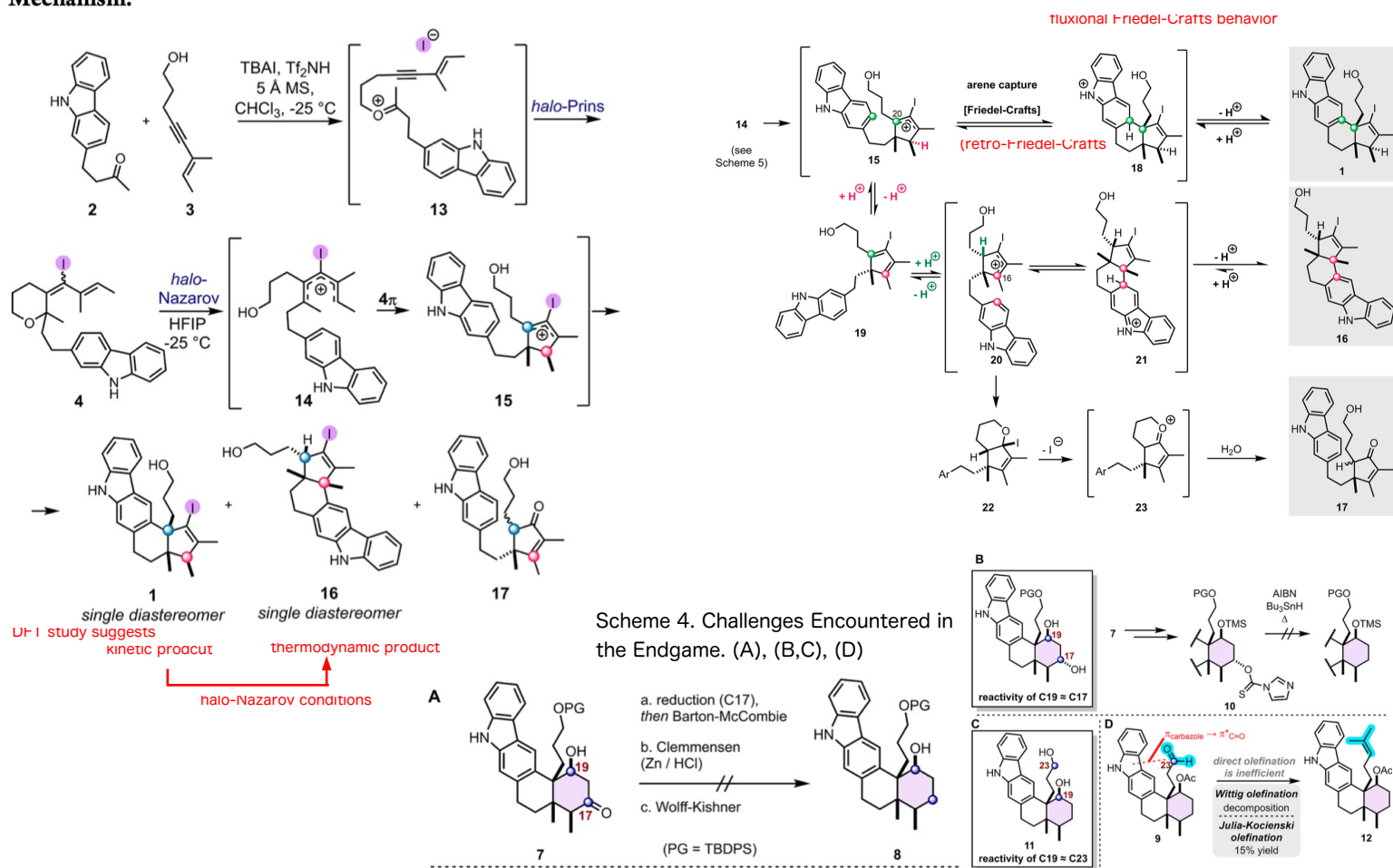
Scheme 5. Halo-Prins/Halo-Nazarov Cationic Cascade Mechanism.
