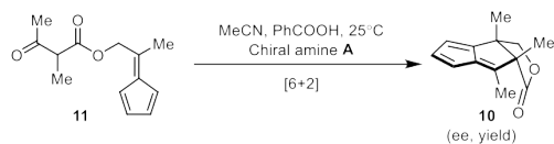
Chiral amine
