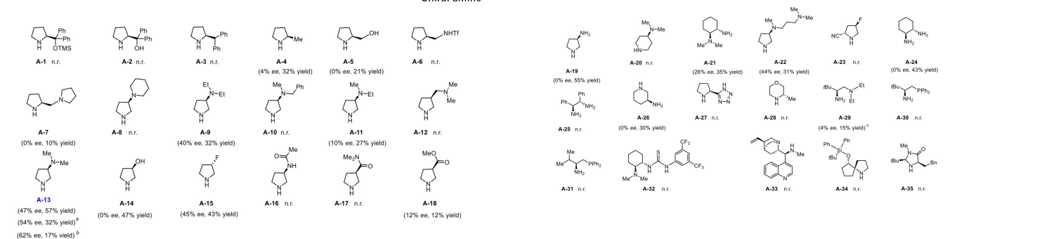
Chiral amine
