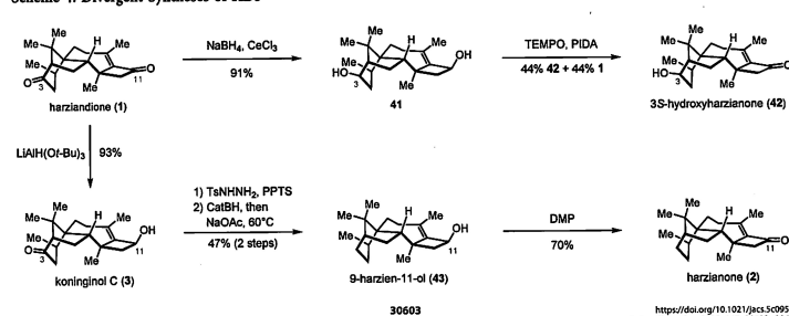
Scheme 4. Divergent Syntheses of HDs
