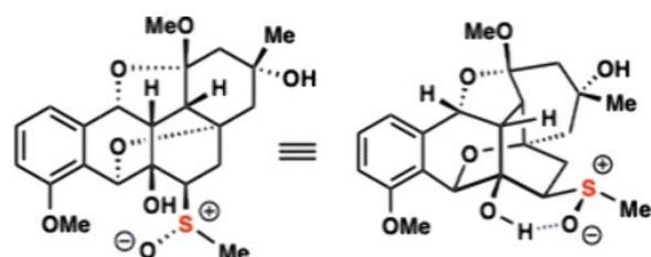
grisemycin thioangucycline polyketide
