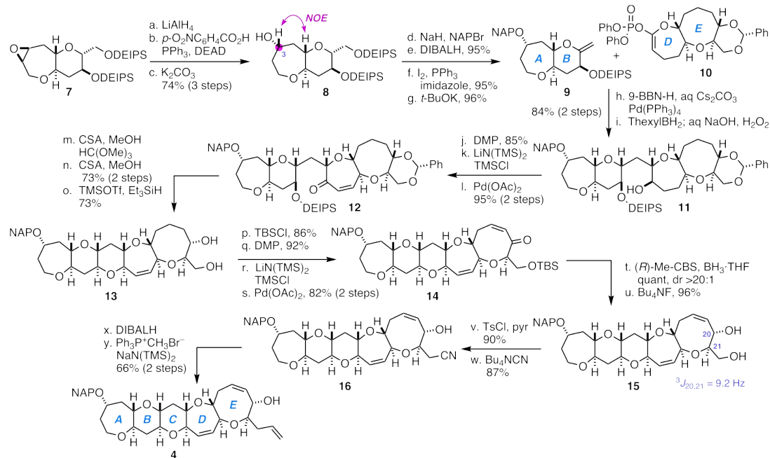
Scheme 2. Synthesis of the C3-Corrected ABCDE-Ring Fragment a
