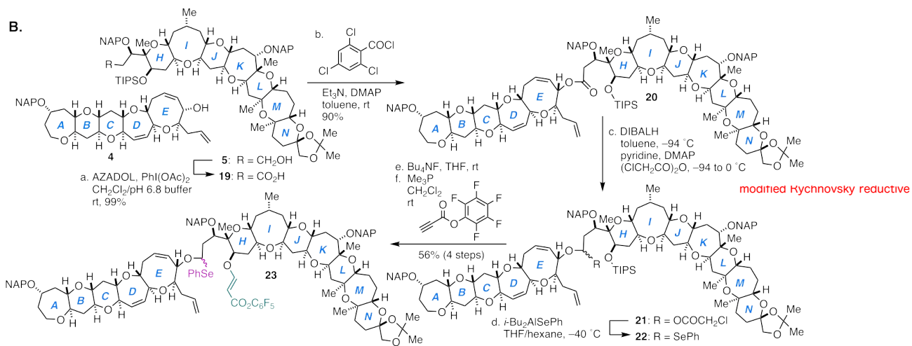
Scheme 4. Total Synthesis of C-CTX1 (1)
