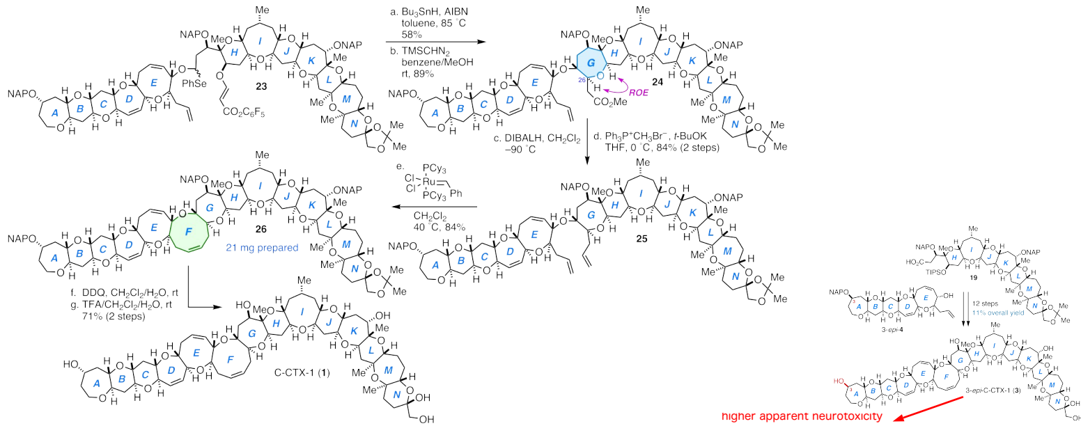
Scheme 4. Total Synthesis of C-CTX1 (1)
